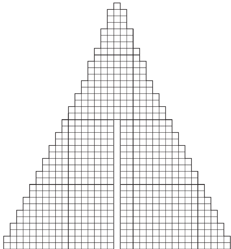
Large Tree Top 35 holes x 38 holes Cut 1
