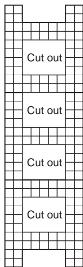
Box Car Ladder 9 holes x 30 holes Cut 2
