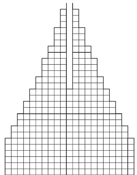
Medium Tree Bottom 21 holes x 28 holes Cut 1
