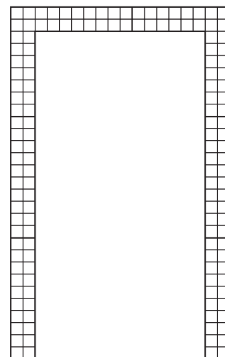
Caboose Door Frame 18 holes x 29 holes Cut 2
