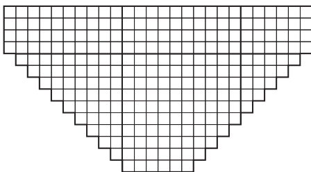
Engine Cow Catcher 26 holes x 14 holes Cut 1
